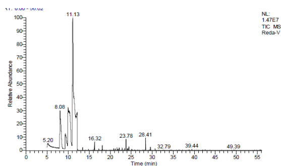
Fig (1): GC/MS chromatogram of orange peels volatile oil.
