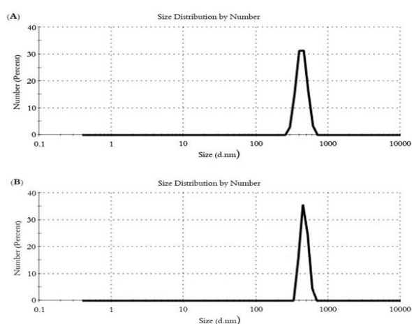
Fig. 3. Nano-formulations particle size (A) ZnO with a size of 433.2 \pm 19.46 nm; (B) ZnO + Citrus cinensis nanoparticle formulation with a size of 458.4 \pm 21.23 nm
