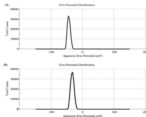
Fig. 4. Nano-formulations zeta potentials (A) ZnO with a zeta potential value of -47.6; (B) ZnO + Citrus cinensis formulation with a zeta potential value of -31.9
